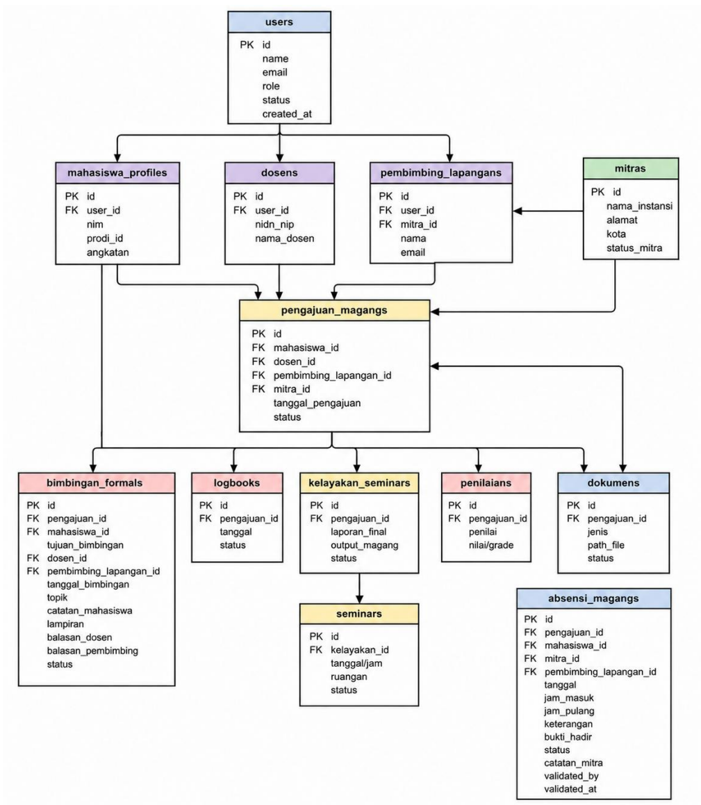
Gambar 7. Entity Relationship Diagram Sistem Informasi Magang
